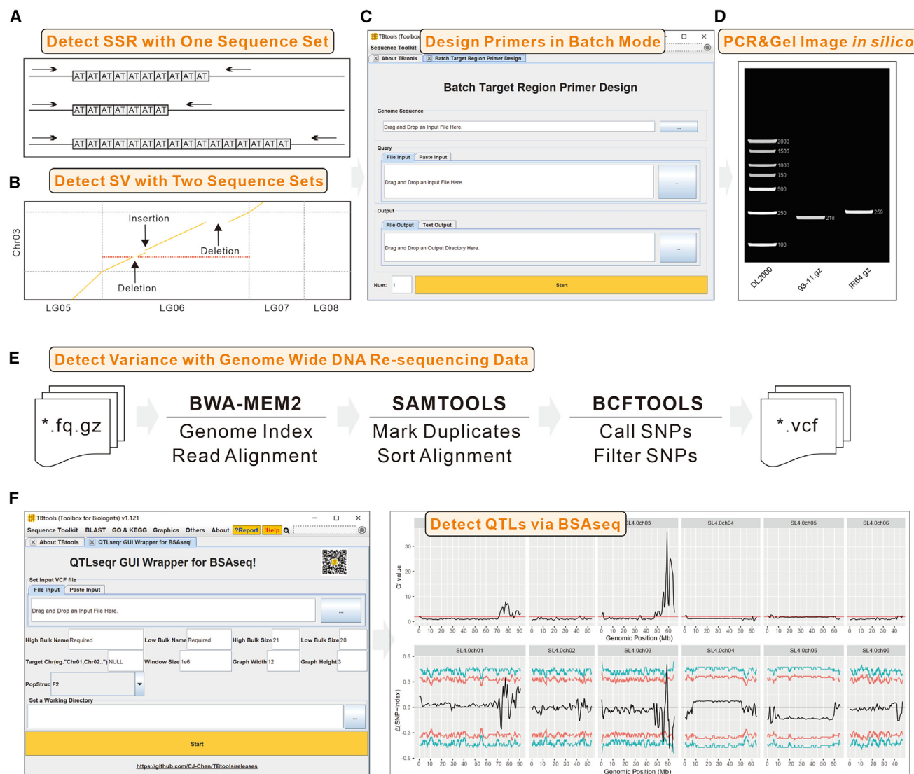
Figure 3. Advanced plugins for post-genomics data analysis in TBtools-II.
